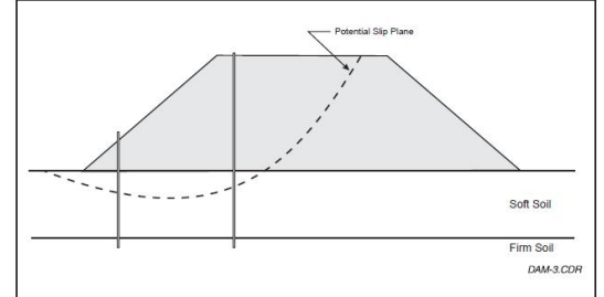
Embankments
