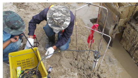
Fig.8 Example of application Measure the lateral movement of pile by inclinometer during Static lateral pile load test.
