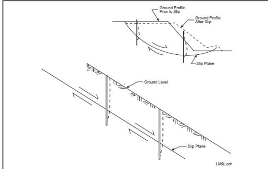
Embankments
